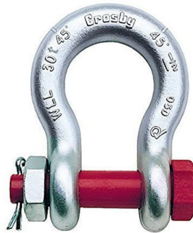
Bow Shackles
